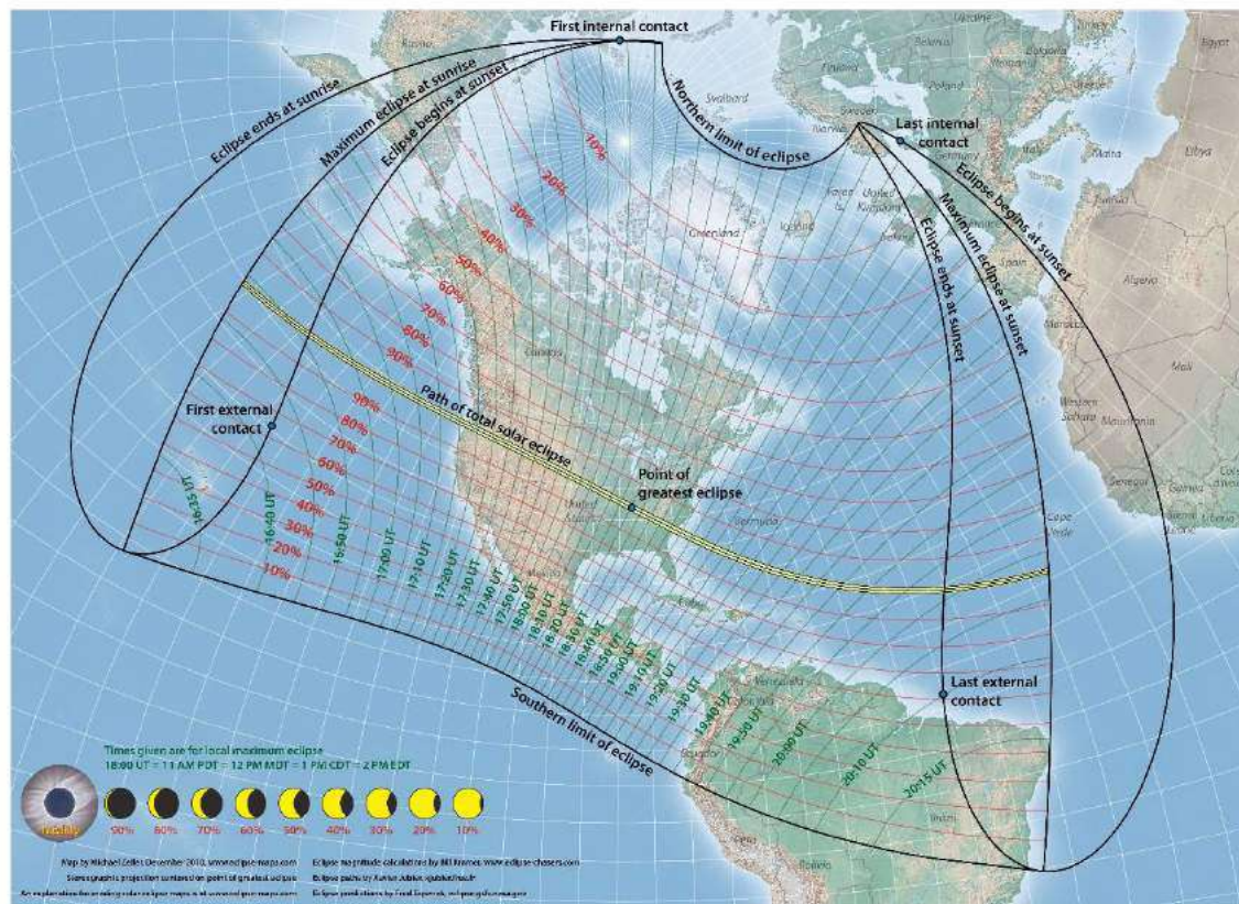
Total Solar Eclipse of 2017 August 21
